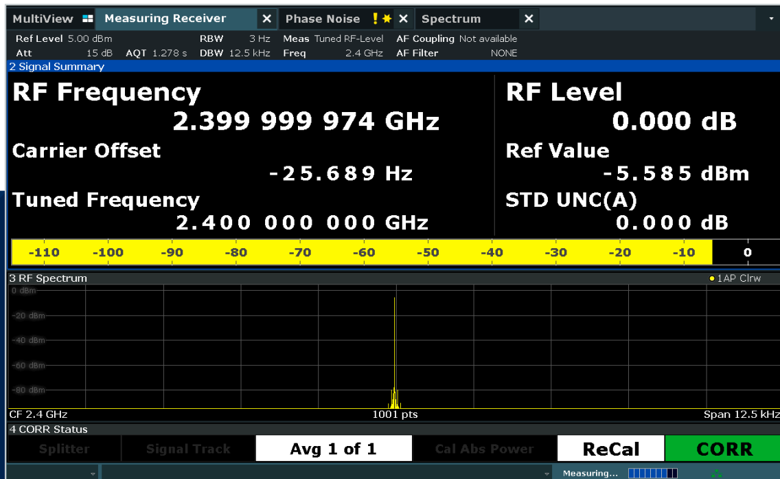
Tuned RF level measurement (TRFL) at 2.4 GHz.
