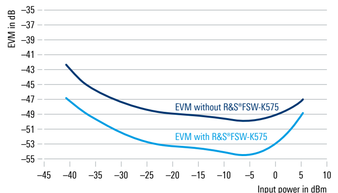
Residual EVM over signal power for a 320 MHz Wi-Fi® IEEE 802.11be signal at 6.905 GHz (modulation order 4096QAM)
