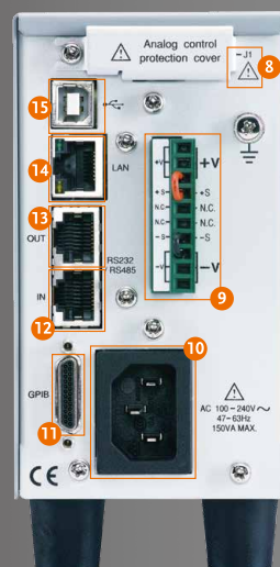
PFR-100M后面板
